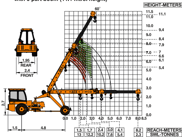
HY-130 Model Crane fitted with 3 part boom (11.1 mtrs. height)
