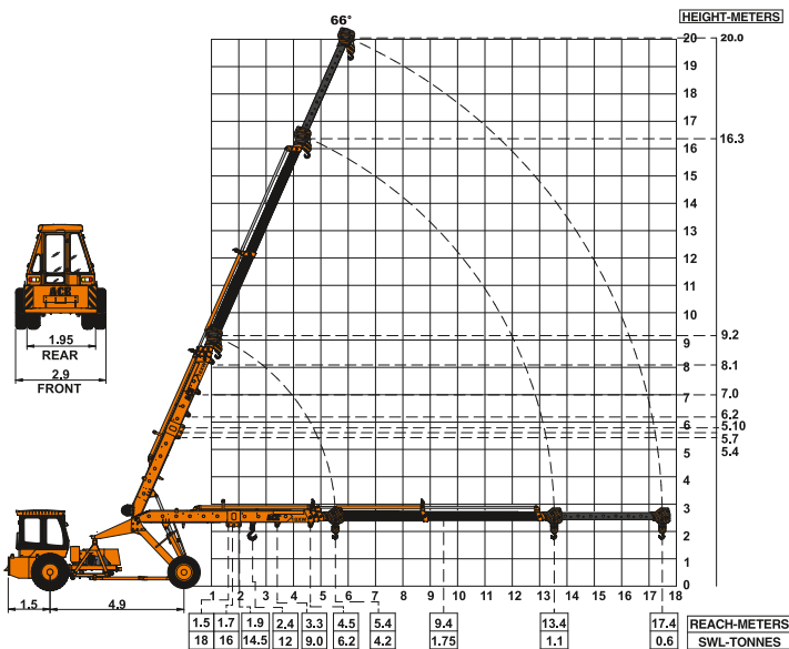
ACE 18XW 4-Part Boom (20 Mtrs. Height) Max. Capacity Manual Extension : 2 Tonnes
